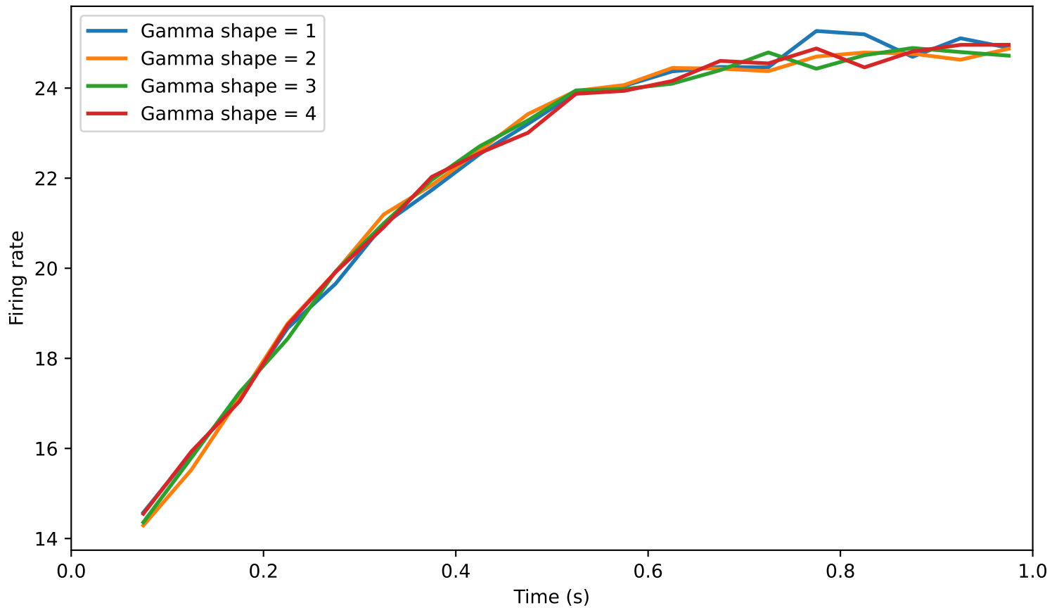
PSTH for ramp model: \beta = 1.1 , \sigma = 0.3
